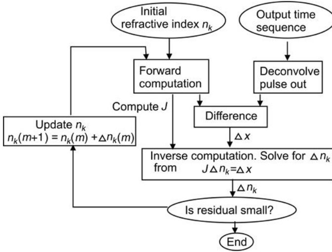
FIGURE 6.20 Block diagram for inverse computation for inspection of unopened packages.
