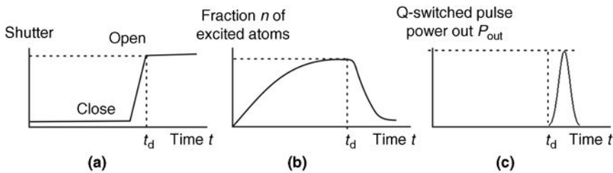
FIGURE 9.4 Timing for Q-switched laser: (a) shutter, (b) fraction of excited atoms at the upper level and (c) output pulse.
