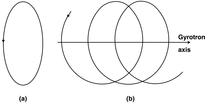
FIGURE 10.3 Resulting trajectory of electron in gyrodevice: (a) transverse circular trajectory and (b) resulting helical trajectory combines \mathbf{v}_{\parallel} and transverse circular.
