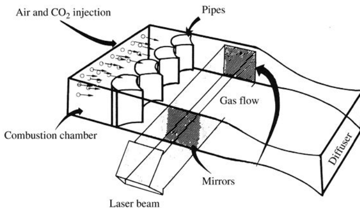
FIGURE 8.8 Structure of a gas dynamic laser.
