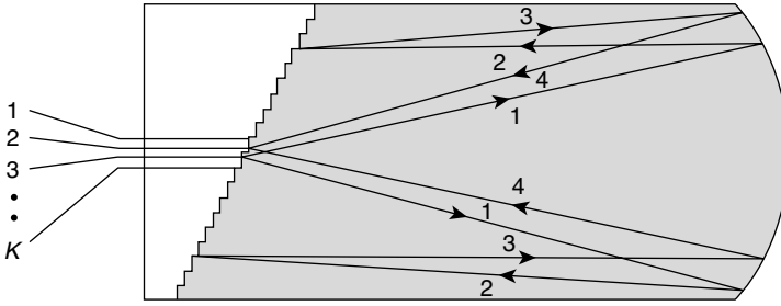
FIGURE 15.5 Device using Littrow condition grating.
