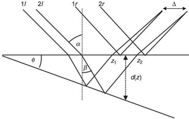
FIGURE 14.4 Fizeau interferometer.
