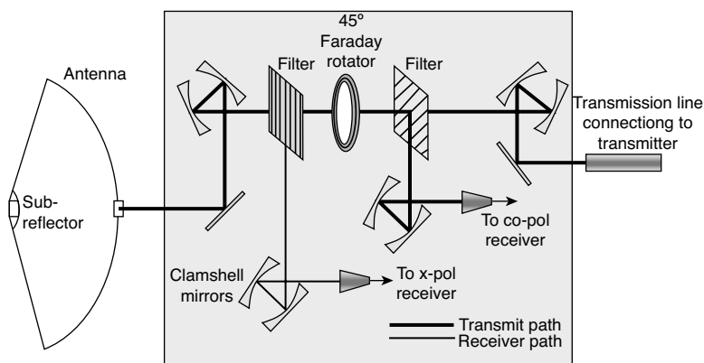
FIGURE 16.6 Quasi-optical duplexer.
