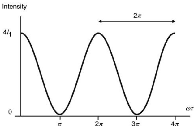
FIGURE 6.2 Output of Michelson interferometer.
