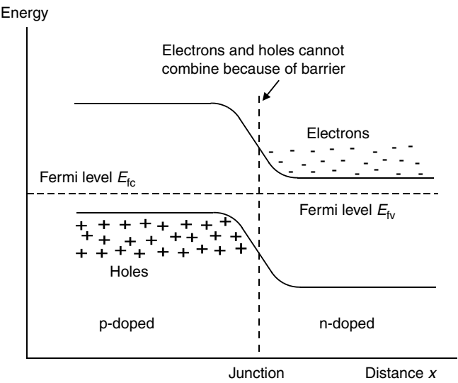
FIGURE 7.5 Semiconductor laser diode with no bias.
