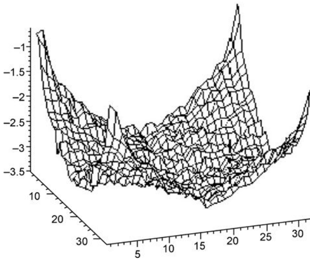
FIGURE 5.8 Average of absolute value of Fourier transform of 10 phase screens produced using the spectral method.
