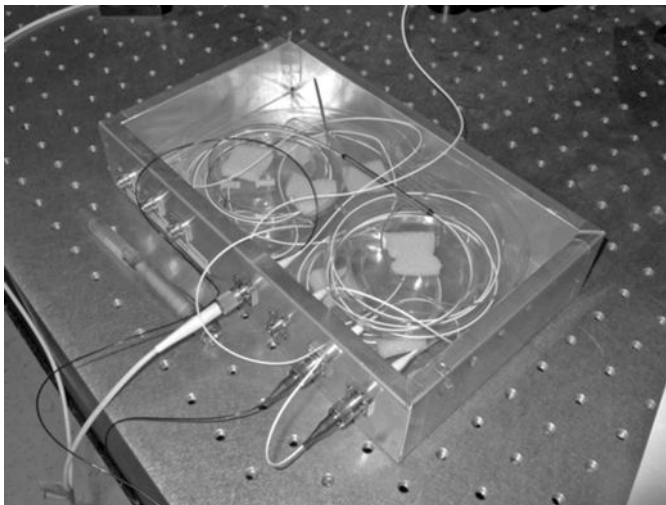
FIGURE 6.7 Laboratory prototype of an optical fiber Mach–Zehnder interferometer.
