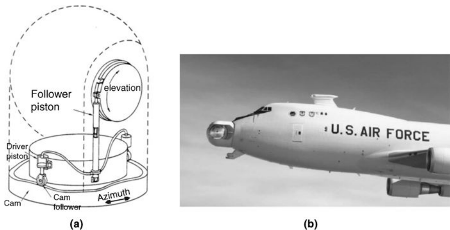
FIGURE 12.7 Rotating turret of airborne laser: (a) mechanism for pointing and tracking and (b) looking sideways.
