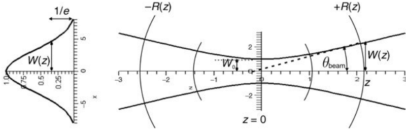
FIGURE 2.1 Gaussian beam propagation.
