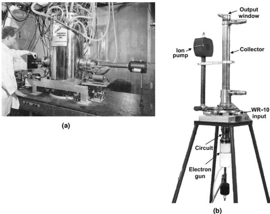
FIGURE 16.5 Photographs of NRL gyrokystron: (a) prototype with cryogenic superconducting magnet and (b) that without superconducting magnet.
