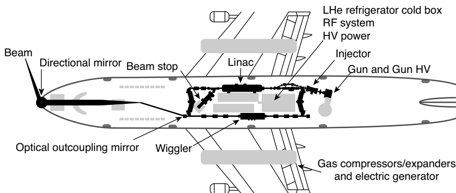
FIGURE 11.2 Layout of free-electron laser on an aircraft.
