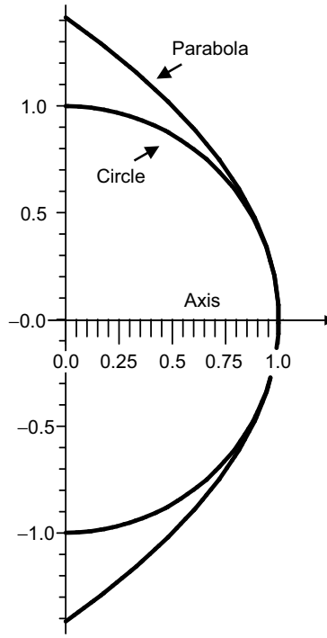
FIGURE 1.1 Illustrates the paraxial approximation.
